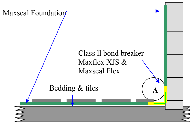
Typical bathroom waterproofing detail for concrete and masonry surfaces
